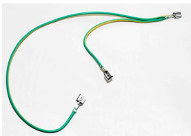
CAB031 3-spade metal case earthing cable
