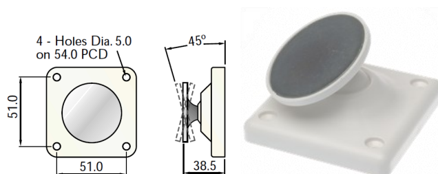
KP02 Universal Keeper Plate
