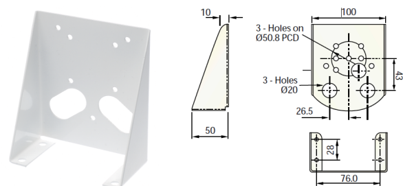
FMB-04 Floor Mounting Bracket
