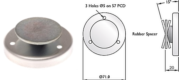
KP01 Metal Keeper Plate
