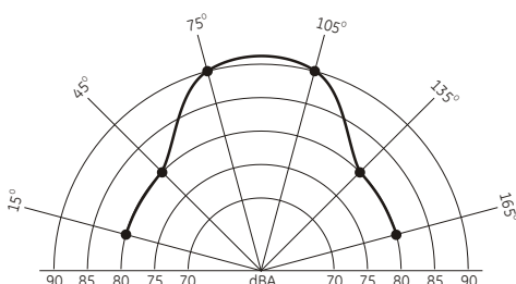
Figure 7: Anechoic sound levels
