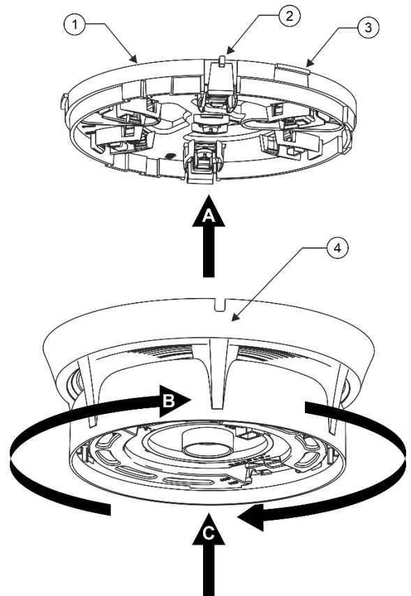
Figure 5: Mounting the sounder
